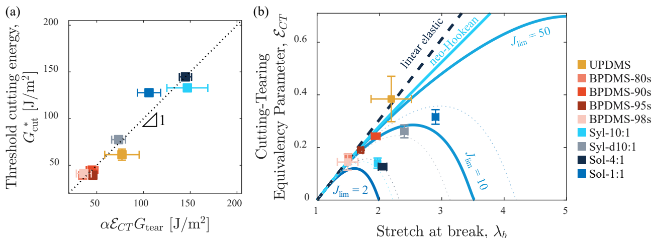
Fig. 5 Mapping cutting and tearing using the equivalency parameter, \mathcal{E}_{CT} . (a) Cutting energy is linearly proportional to the product of tearing energy and \mathcal{E}_{CT} for the hyperelastic silicones tested. The fit constant \alpha = 7.2 allows the data to be plot on a zero intercept line of slope one (black dotted). (b) A plot of \mathcal{E}_{CT} versus the stretch at break \lambda_b for a linear elastic material (dark dashed line), neo-Hookean (teal line), and a Gent material with decreasing limiting stretch (decreasing J_{lim} corresponds to increasing color saturation). Experimentally-determined \mathcal{E}_{CT} and \lambda_b values are provided for comparison. For Sol-1:1, Sol-4:1, Syl-10:1, and Syl-d10:1, a corresponding Gent behavior line (dotted line) is added using J_{lim} determined from a fit to the response in Fig. 2a. Error bars are determined from the standard deviation of three or more samples. The legend at the right applies to both plots.
