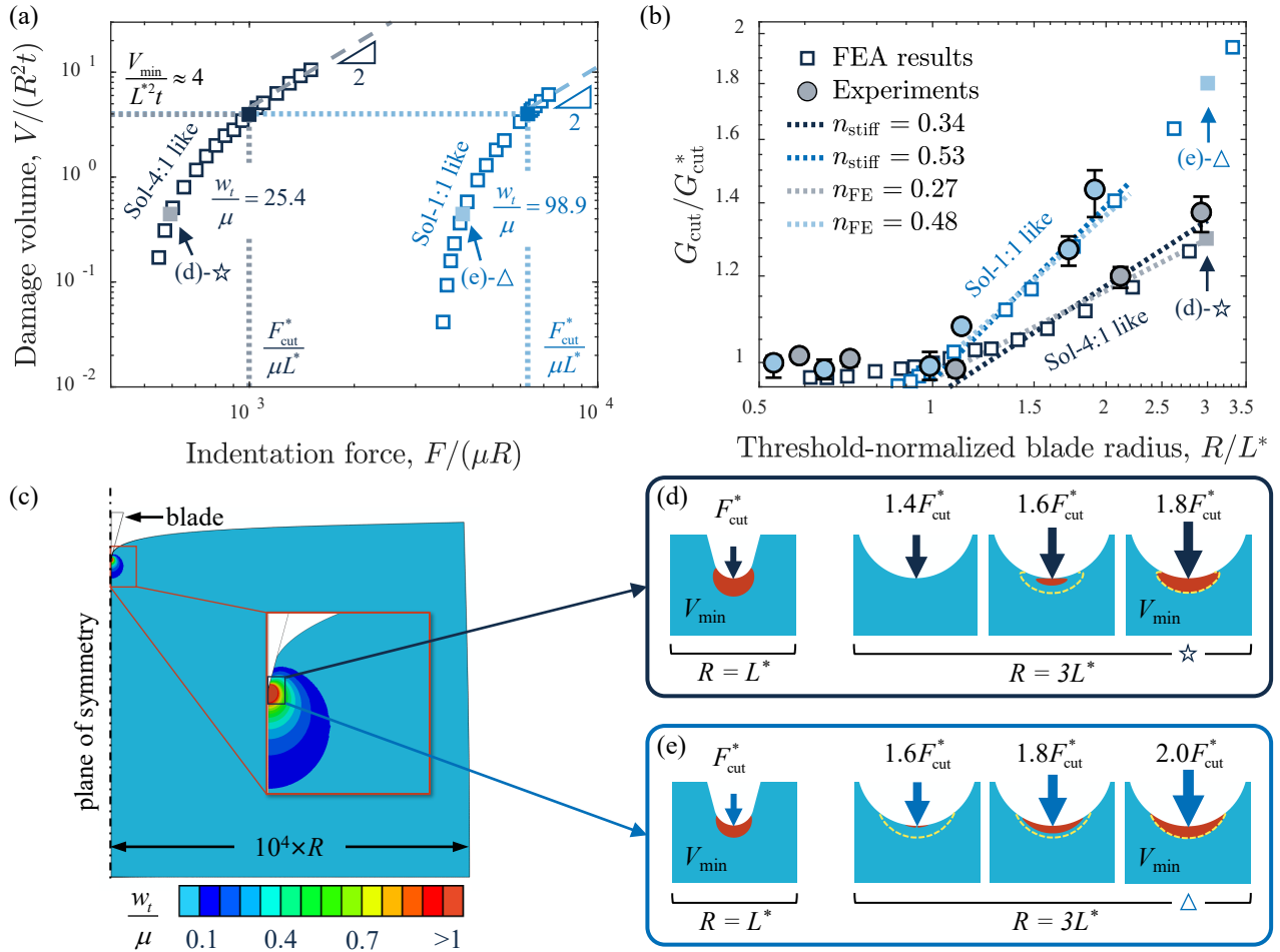
Fig. 7 Using a minimum damage volume to predict the radius-dependence of G_{\text{cut}} . (a) The relationship between normalized damage volume V/(R^2t) and normalized force per unit thickness F/(\mu R) as obtained from FE simulation of a blade indenting a hyperelastic Arruda-Boyce half-plane. The threshold strain energy density w_t/\mu used to determine the volume was selected such that at V_{\min}/(L^2t) \approx 4 the normalized force per unit thickness matches that observed experimentally (filled solid squares and dotted lines) for either a Sol-4:1 like material (dark blue) or a neo-Hookean Sol-1:1 like material (light blue). Light-colored solid squares mark V_{\min}/(L^2t) \approx 4/9 and the F/(\mu R) that correspond to R = 3L^* for each material as shown in parts (d) and (e). (b) The force predictions in (a) are converted to normalized cutting energy G_{\text{cut}}/G_{\text{cut}}^* according to Eqn. (1) to illustrate the radius dependence of the cutting energy. Power law fits of the cutting energy increase predicted by FE ( n_{\text{FE}} , light dotted lines) compare favorably with those determined experimentally ( n_{\text{stiff}} , darker dotted lines). Experimental data from Fig. 2 is shown for comparison (circles). Light-colored solid squares again correspond to R = 3L^* as shown in parts (d) and (e). (c) FE illustration of a blade indenting a half-plane. The size of the FE half-plane is approximately four orders of magnitude larger than the blade radius. A dash-dotted line indicates the plane of symmetry. Inset: a close-up of the near-tip strain energy density field, normalized by the shear modulus. (d) and (e): FE visualization of the evolution of the threshold damage volume as a function of radius R and cutting force: (d) Sol-4:1 like and (e) Sol-1:1 like materials. In both examples, the left image corresponds to the onset of the threshold cutting regime R = L^* , which requires force F_{\text{cut}} and defines V_{\min} . The radius is tripled in the right images, requiring a force larger than the threshold value for the damage zone (red region) to attain V_{\min} . Correspondence with parts (a) and (b) are indicated by star and triangle symbols for the Sol-4:1 like and Sol-1:1 like responses, respectively.
