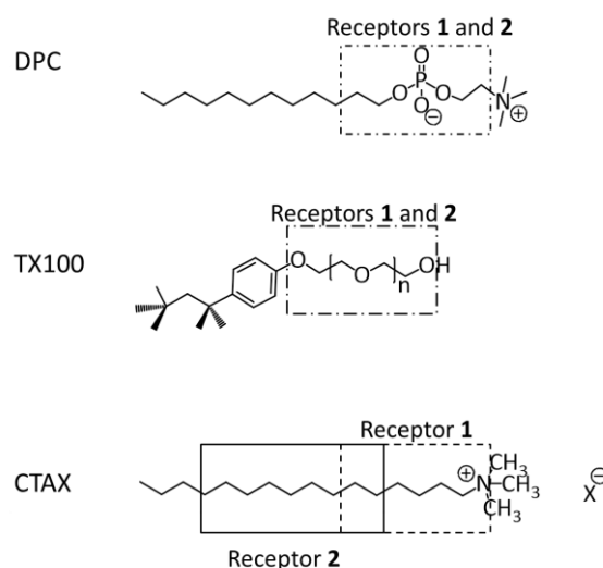
Figure 4. Schematic representation of the localisation of the receptor within the different types of micelles
