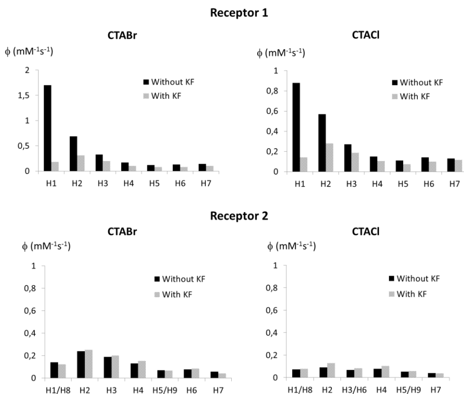
Figure 5. Normalized relaxivity values for the protons of receptors 1 (top) and 2 (bottom) solubilized in 50 mM CTABr micelles (left) and 50 mM CTACl micelles (right) before and after addition of 4 equivalents of KF. All normalized PRE are given in the SI.
