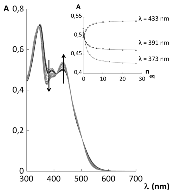
Figure 2. UV-vis titration of a 5.05 \cdot 10^{-5} M solution of receptor 2 in 50 mM CTABr with KF and the 1:1 binding isotherms with parametric adjustment.
