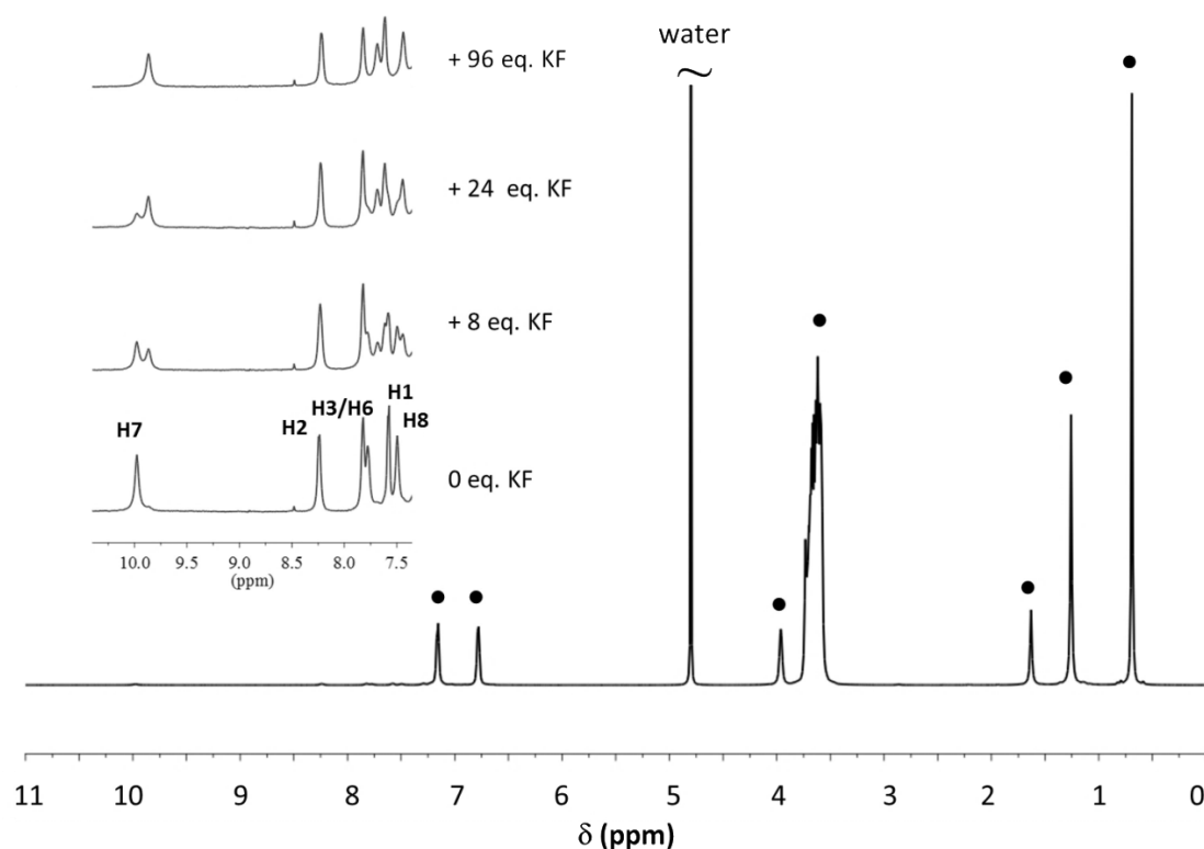
Figure 3. ^1\text{H} NMR spectrum of a 1.5mM solution of receptor 2 in 50 mM Triton X-100. Receptors signals are amplified and shown for different additions of KF. (●) surfactant signals. The assignment of the receptor signals was made by comparison with the spectrum of the receptor in CTAX micelles. For proton labelling see Figure 1.
