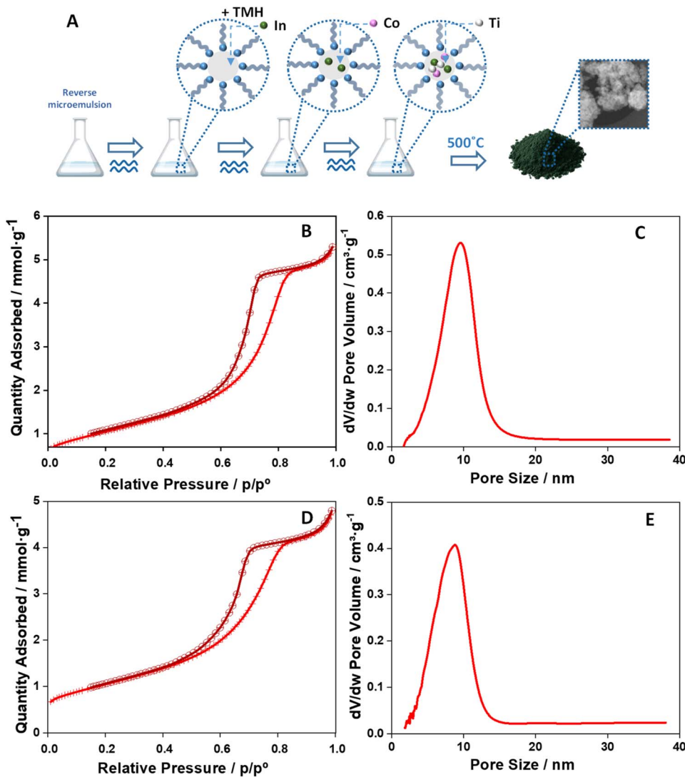
Fig. 1 (A) Schematic representation of the synthesis carried out using the reverse microemulsion method. (B) Nitrogen adsorption–desorption isotherm results for the 2.5In–Co–Ti sample. (C) Pore volume distribution for the 2.5In–Co–Ti sample. (D) Nitrogen adsorption–desorption isotherm results for the 10In–Co–Ti sample. (E) Pore volume distribution for the 10In–Co–Ti sample.
