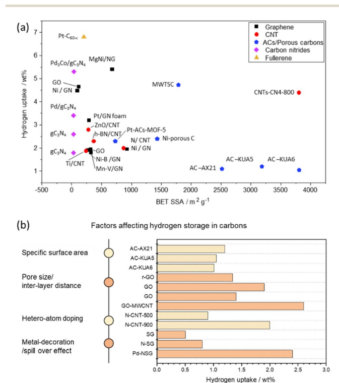
Fig. 7 (a) Comparison of the H 2 storage capacities of carbon-based adsorbents with respect to their specific surface area and (b) factors affecting the hydrogen storage in carbon-based materials.
