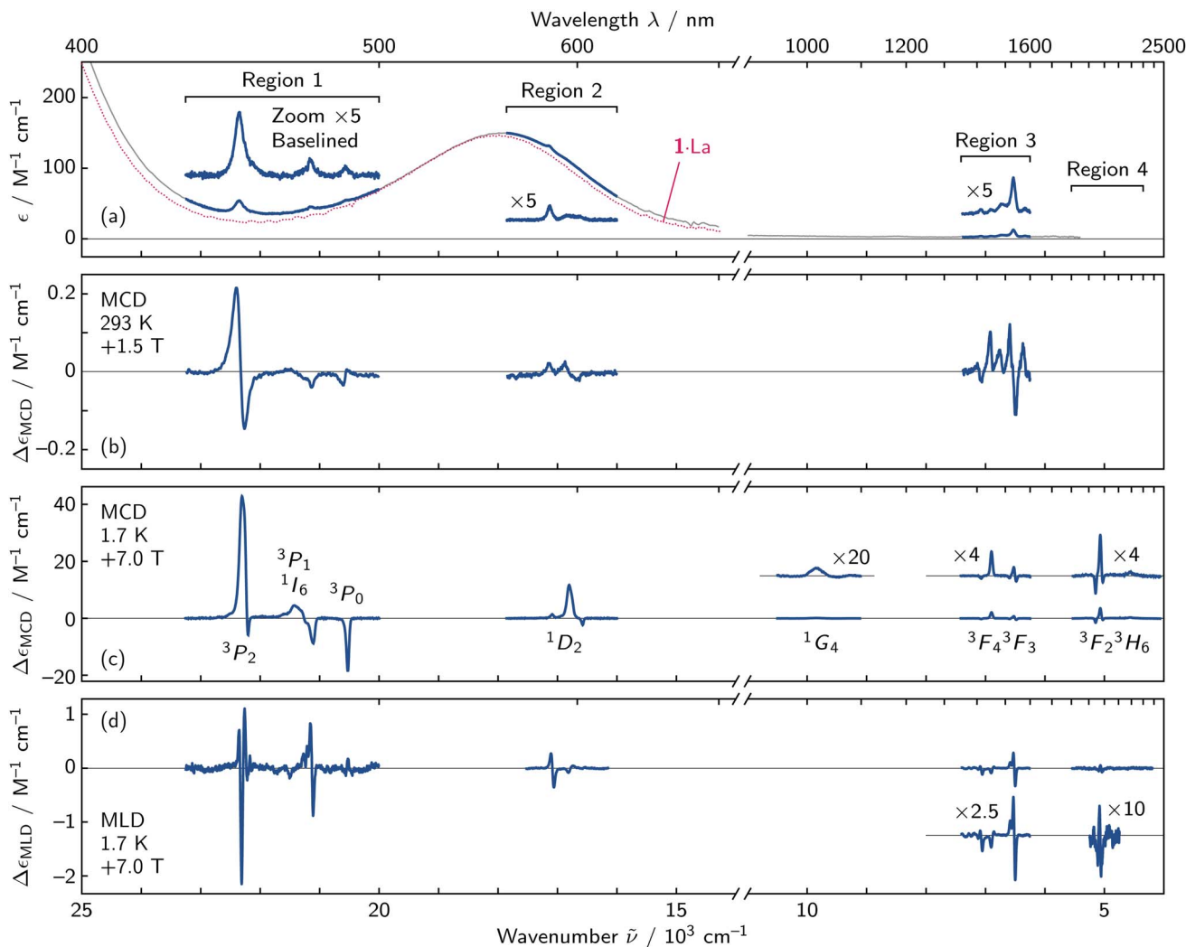
Fig. 4 (a) Absorption, (b) and (c) MCD, and (d) MLD spectra of 1-Pr are shown at various temperatures. Regions of interest are shown in blue and labeled, and an absorption spectrum of 1-La is included for comparison. There are no data within region 4 in the room temperature spectra due to the strong absorption of the solvent.
