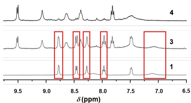
Figure 2: 1 H-NMR spectra of 1 , 3 and 4 (300 MHz, d 6 -DMSO, 298 K). For clarity, only the aromatic region is shown here.
