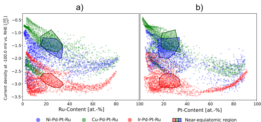
Fig. 6 Comparative HER activity plot from which correlations between the Ru-content (a) and the Pt-content (b) with the HER activity (indicated by the current density at -100 mV vs. RHE) can be inferred. The colour-coded markers show all compositions of the HER dataset. The near-equiatomic compositions (all constituents between 15 and 35 at%) of each system are framed. In the Pt-richest compositions a decrease in activity is observed in the Ir-Pd-Pt-Ru system (red). The Ru-richest compositions show a decreasing activity trend in all systems.
