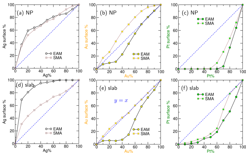
Fig. 1 Surface fractions in selected elements, as the overall concentration of this element is increased in 4033-atom nanoparticles (upper panels) or 4032-atom (111) slabs (lower panels), predicted from the EAM and SMA potentials. The dashed blue line is the expected result for the ideal solid solution. (a and d) Ag; (b and e) Au; (c and f) Pt.
