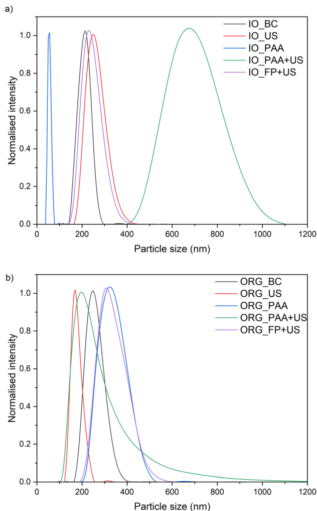
Fig. 4 Particle size distributions of LNP and base-case lignins from (a) ionosolv treatment, and (b) organosolv treatment.
