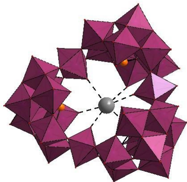
Figure 8. Structure of [M\{-\{\beta\text{-As}^{\text{III}}\text{W}_8\text{O}_{30}\}(\text{WO}(\text{H}_2\text{O}))_3\}_3]^{14-} with the central guest being either \text{K}^+ or \text{Rb}^+ . Color code: \text{WO}_6 (violet octahedra), As (orange), K/Rb (grey). 114
