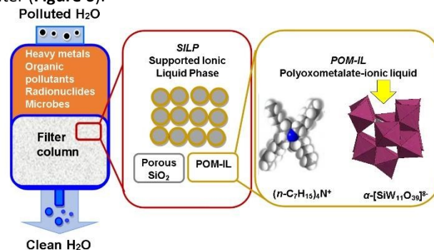
Figure 6. Water purification using POM-SILPs: the POM-SILP column filter removes toxic heavy metals (e.g. Ni(II) , Pb(II) , UO_2(II) ), microbes ( E. coli ), and aromatic organic pollutants (e.g. trityl dyes) due to the presence of lacunary polyoxometalate anions with specific metal-binding sites (yellow arrow) and antimicrobial tetra-alkyl ammonium cations. Reproduced from Ref. 63 with permission from Wiley-VCH, Copyright 2017.
