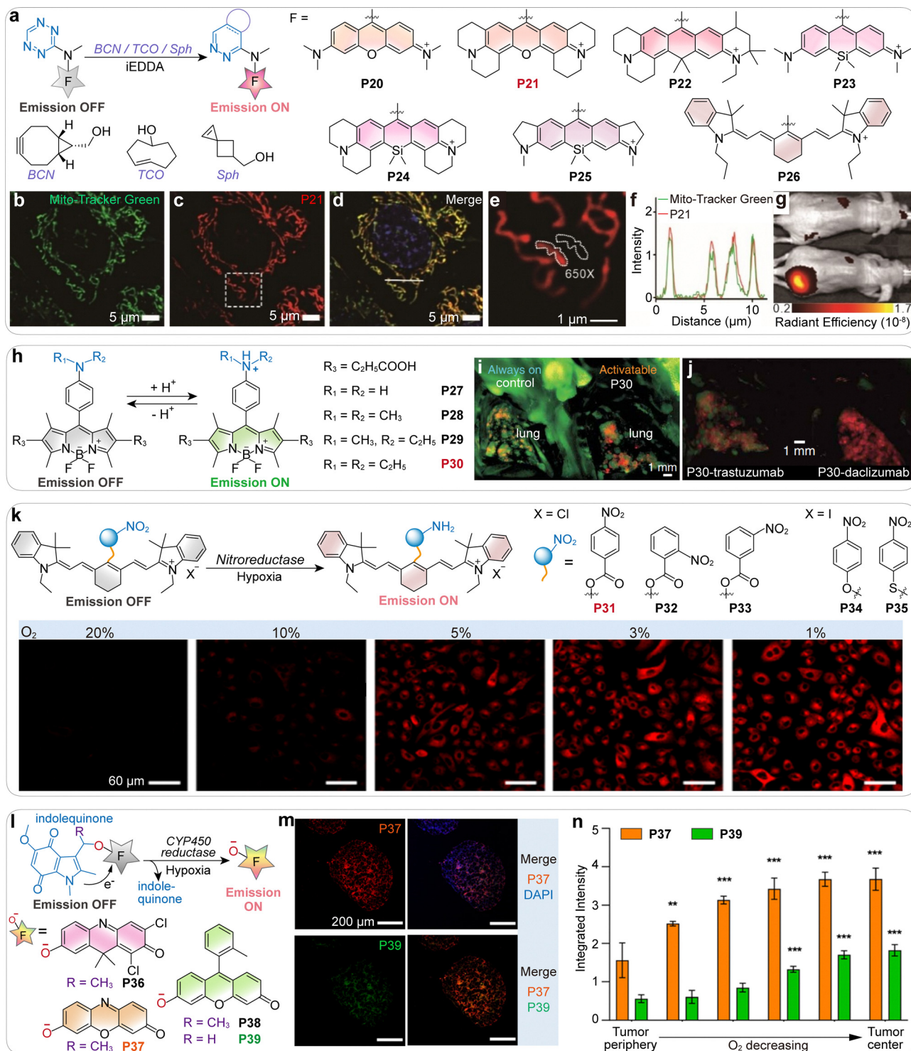
Fig. 10 (a) Fluorogenic reactions between tetrazine probes P20–P26 and dienophiles. (b)–(d) Colocalization imaging of mitochondria using Mito-Tracker Green (green) and P21 (red). Scale bars: 5 \mu\text{m} . (e) Comparison of pixel intensity between regions of interest located within and outside mitochondria, in the boxed area shown in panel (c). Scale bar: 1 \mu\text{m} . (f) Plot of fluorescence intensity along the white line shown in panel (d). (g) In vivo imaging of mice using P22 . Mice bearing tumor xenografts were intratumorally injected with saline (top) or TCO-TPP (bottom), followed by administration of P22 after 5 min. (h) The reversible and acidic pH-induced fluorescence activation of P27–P30 . (i) Composite overlapped images of the mouse lung 1 day after injection of always-on probe (left) and pH-activatable probe P30 (right). (j) Spectrally unmixed and composite overlapped images of the lung 1 day after injection of pH-activatable antibody probes. Left: HER2-specific probe ( P30 -trastuzumab) selectively highlights HER2 + tumors (green) in the lung, clearly distinguishing them from RFP-labeled HER2 - tumors (red). Right: Control probe ( P30 -daclizumab, targeting CD25) shows no green signal, indicating a lack of HER2 + tumor labeling; only RFP + HER2 - tumors (red) are visible. This comparison demonstrates that fluorescence activation occurs only when the probe binds and is internalized by HER2 + cells, confirming the probe's target specificity and pH-dependent activation. (k) Oxygen-dependent nitroreductase-activated fluorescence turn-on of probes P31–P35 , and the confocal fluorescence microscopy
