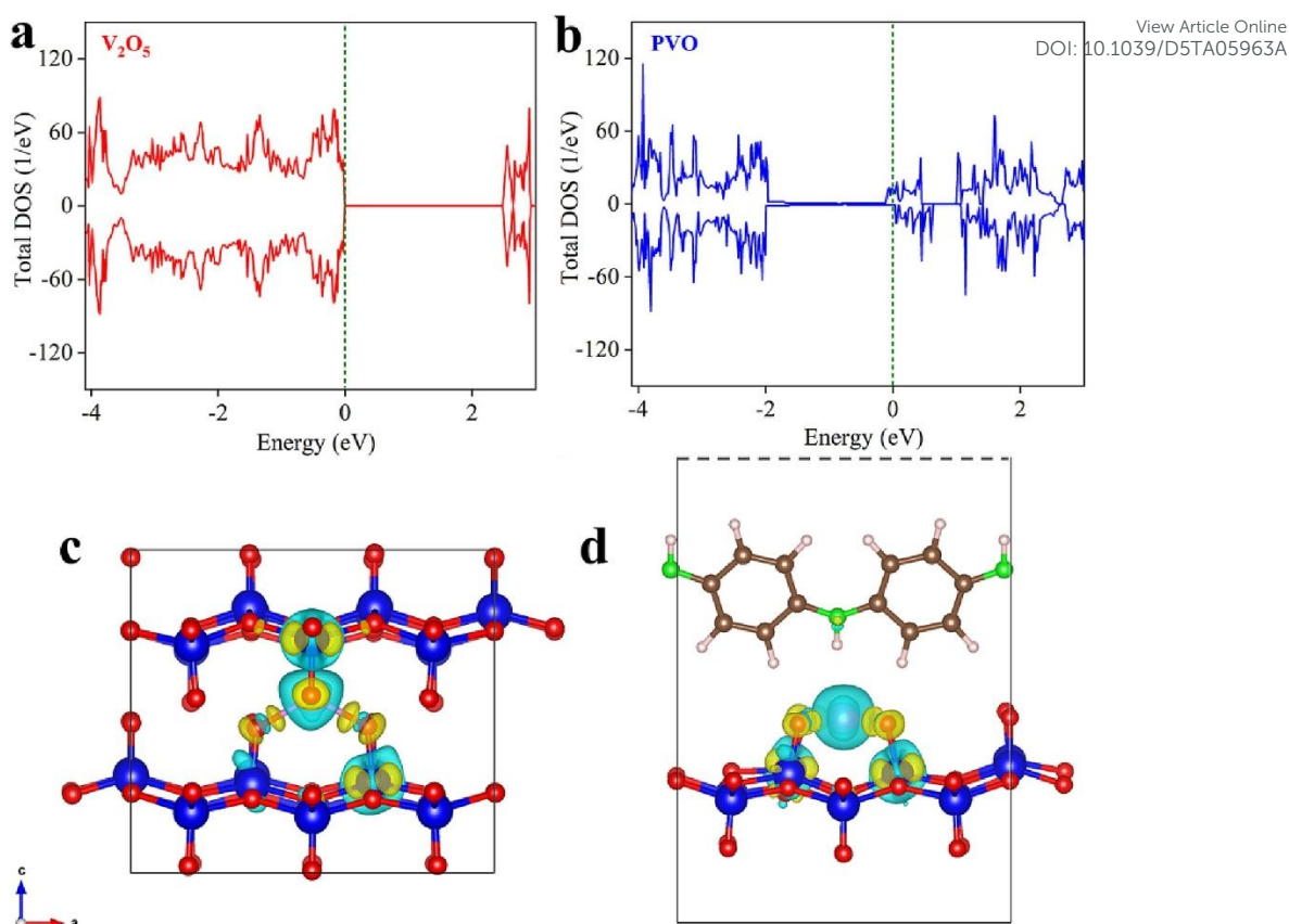
Figure 6. Total density of states for (a) pristine V_2O_5 and (b) PVO (V-MOF-derived hierarchical porous V_2O_5 ). (c, d) Differential charge density with Zn^{2+} intercalation in V_2O_5 and PVO. Color code: blue, red, brown, green, purple, and white balls represent V, O, C, N, Zn, and H atoms, respectively. Reprinted from Ref. [68], copyright (2023), with permission from Elsevier.
