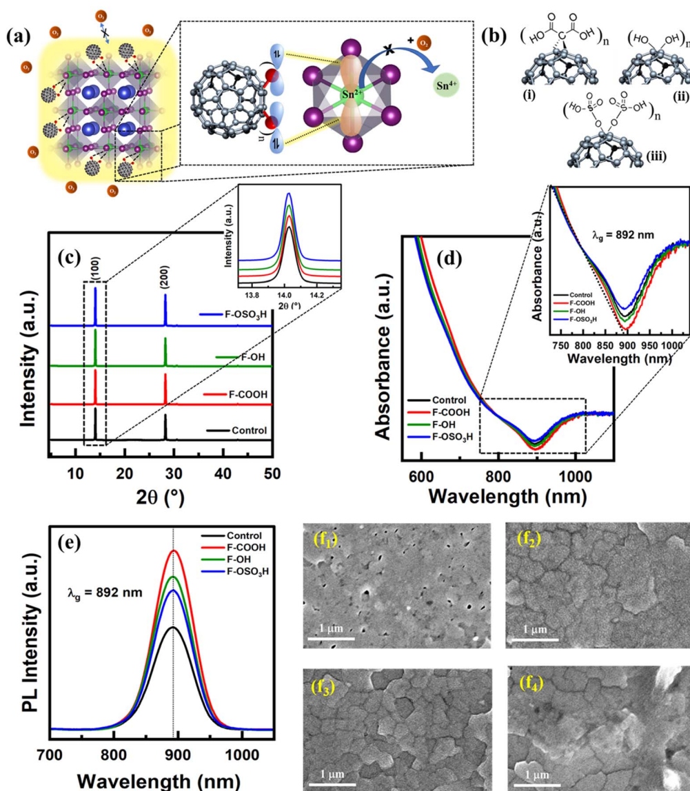
Fig. 1 (a) Schematic interaction of fullerene-based additive with Sn-HP. (b) Molecular structure of different additives employed in the study ((i) C 60 (COOH) 2 (F-COOH), (ii) C 60 (OH) 2 (F-OH), (iii) C 60 (OSO 3 H) 2 (F-OSO 3 H)). (c) XRD patterns (with a zoomed view), (d) absorbance spectrum (with a zoomed view), (e) PL spectrum, and (f) SEM images of perovskite film without and with functional additives ((f 1 ) control, (f 2 ) F-COOH, (f 3 ) F-OH, (f 4 ) F-OSO 3 H).
