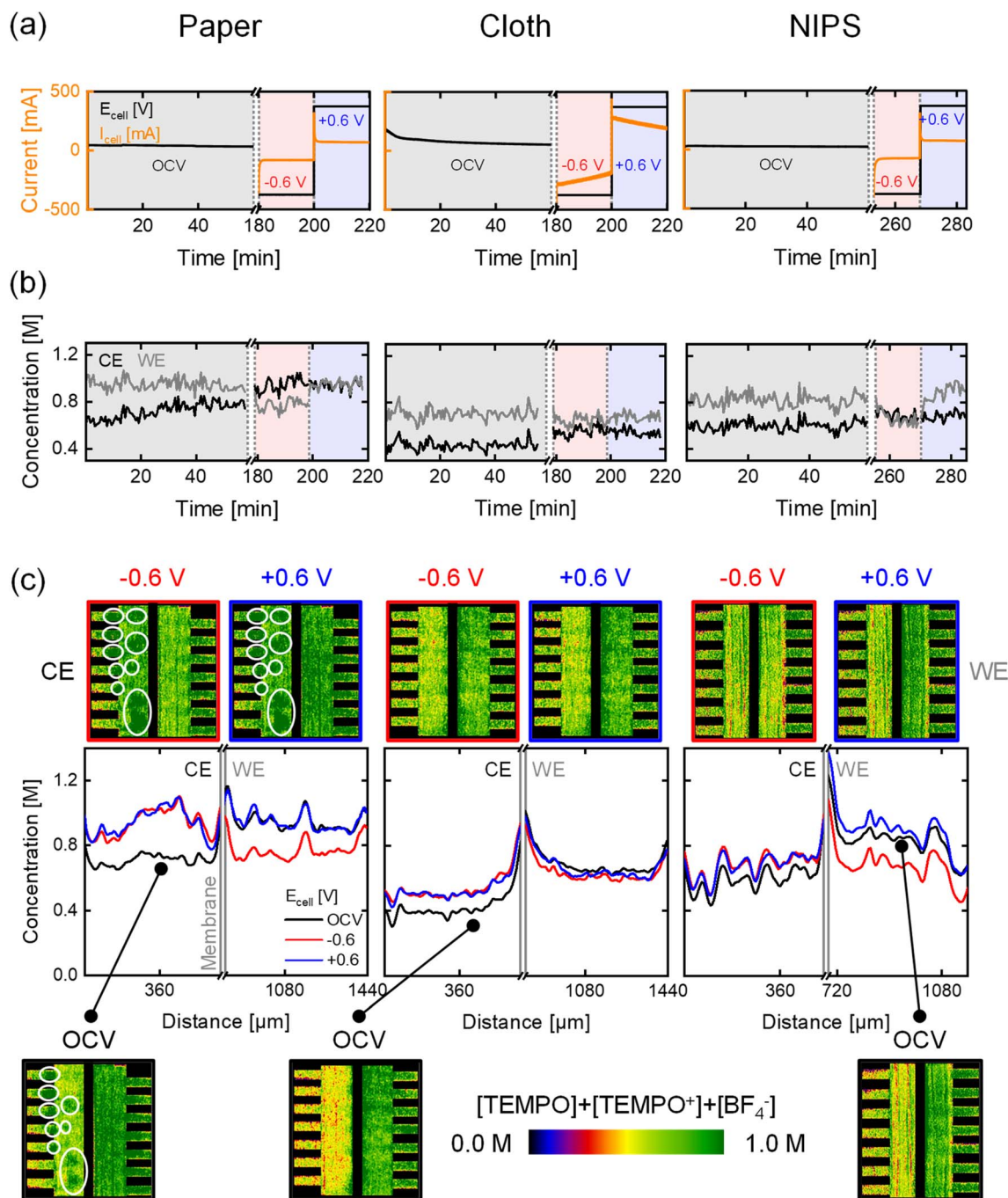
Fig. 3 Operando neutron imaging of the active species transport with the attenuating BF 4 - supporting ion for three electrode types: paper, cloth, and an in-house manufactured NIPS electrode, at an inlet flow rate of 5 mL min -1 and evaluated at OCV, -0.6 V, and +0.6 V. (a) The potential applied and current output of the electrochemical cells. (b) The averaged concentration profiles over time in the counter electrode (CE) and the working electrode (WE). (c) The cumulative active species (TEMPO and TEMPO + ) and BF 4 - supporting ion concentration profiles over the electrode thickness with the averaged snapshots of the cell after image processing, with on the counter electrode 0.5 M TEMPO and at the working electrode 0.5 M TEMPO + BF 4 - . Salt precipitation in the cell is highlighted in the snapshots.
