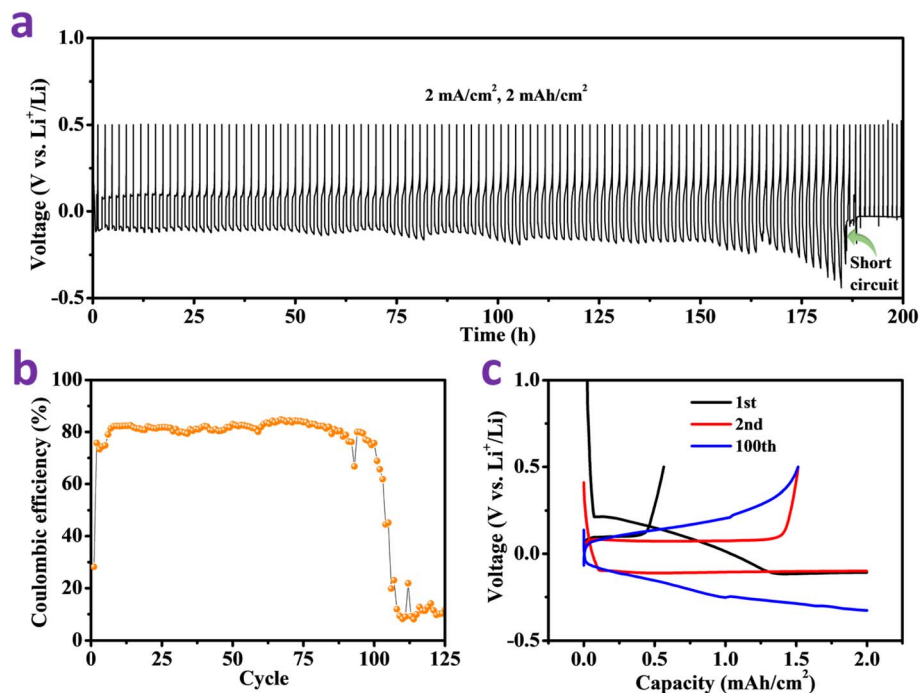
Fig. 3 (a) Cycling performance, (b) coulombic efficiency, and (c) corresponding voltage profiles of lithium plating/stripping on MnO 2 @Cu at a current density 2 mA cm -2 and areal capacity of 2 mA h cm -2 .
