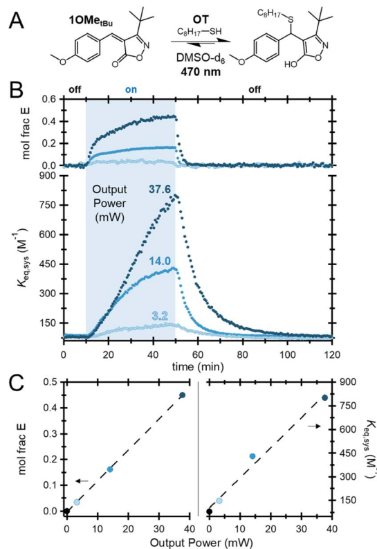
Fig. 5 (A) Equilibrium between 1OMe t Bu and OT. (B) Mole fraction of the Z isomer and overall system K_{eq} ( K_{eq,sys} ) of 1OMe t Bu equilibrated with OT during the NMR photoisomerization experiment at varying LED output powers (3.2 to 37.6 mW). (C) Mole fraction of Z isomer and maximum system K_{eq} versus LED output power.
