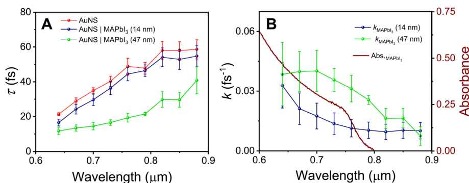
Fig. 3 (A) SPP lifetime versus wavelength for bare AuNS and AuNS coated with \text{MAPbI}_3 . (B) Rate constant for SPP decay ( k_{\text{MAPbI}_3} ) induced by \text{MAPbI}_3 . The red curve shows the steady-state absorption spectra of a \text{MAPbI}_3 film prepared from a concentrated precursor solution (0.4 M). Note that the \text{MAPbI}_3 thin films used in the SPP experiments were prepared from diluted precursor solutions: 20 mM or 40 mM for the 14 nm or 47 nm thick films, respectively. The concentrated film was used here for improved clarity. The error bars correspond to 95% confidence limits.
