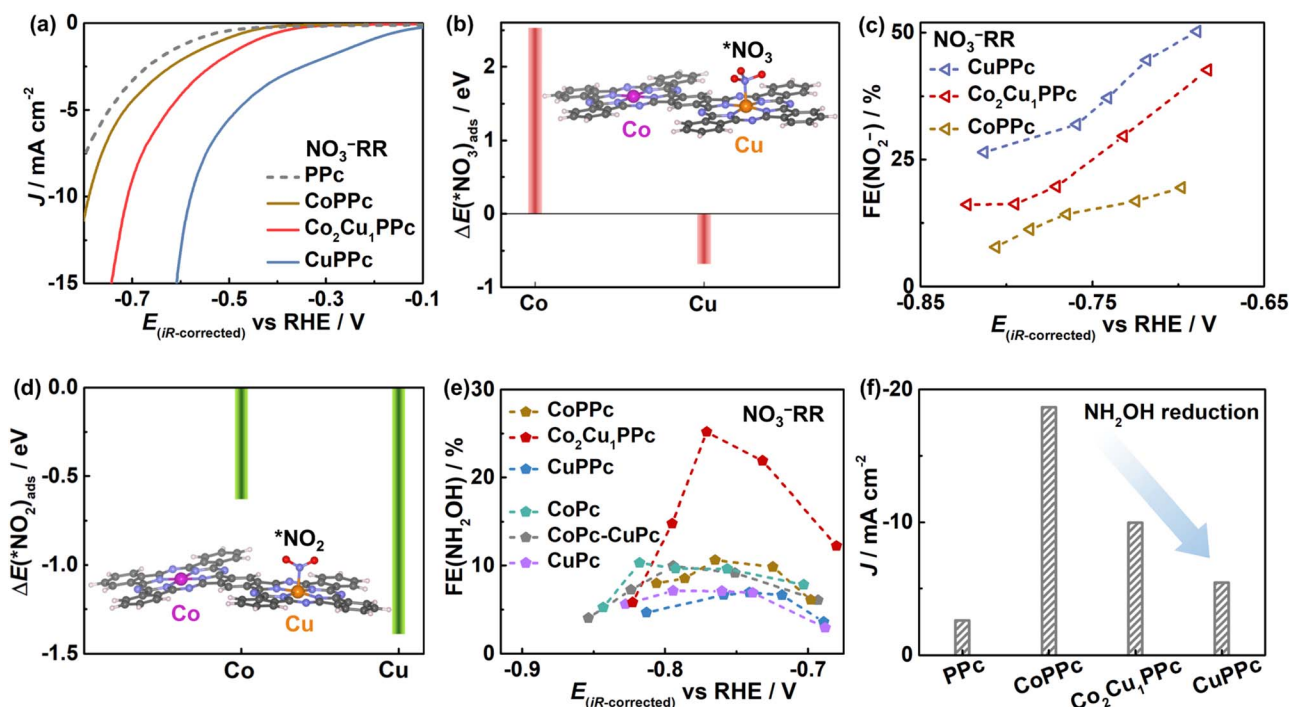
Fig. 3 Electrocatalytic performance for the NO 3 - RR. (a) LSV curves of PPc, CoPPc, Co 2 Cu 1 PPc and CuPPc in Ar-saturated 0.1 M KHCO 3 containing 0.8 M KNO 3 . (b) Adsorption energy of *NO 3 on the Co or Cu sites of Co 2 Cu 1 PPc (inset: the most stable adsorption configurations of *NO 3 ). (c) FEs of NO 2 - formation after the NO 3 - RR with CoPPc, CuPPc, and Co 2 Cu 1 PPc. (d) Adsorption energy of *NO 2 on the Co or Cu sites of Co 2 Cu 1 PPc (inset: the most stable adsorption configurations of *NO 2 ). (e) FE(NH 2 OH) for the NO 3 - RR with CoPPc, CuPPc, Co 2 Cu 1 PPc, CoPc, CuPc, and CoPc-CuPc as a function of potential. (f) Current densities for the side-reaction of NH 2 OH reduction at -0.76 V RHE in 0.1 M KHCO 3 containing 30 mM NH 2 OH.
