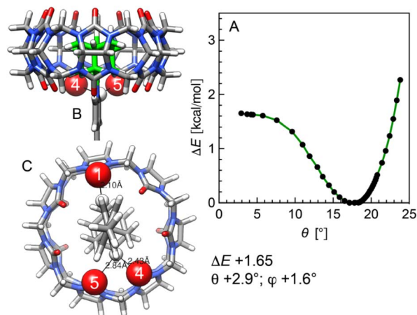
Fig. 8 (A) Relative stability of assembly 12·CB[7] as a function of the CB[7] tilt angle \theta relative to the rod axis. (B) Side and (C) top views of assembly 12·CB[7], with a tilt angle \theta of 2.9°. See Fig. 5 for the description of the angles; relative energies in kcal mol -1 .
