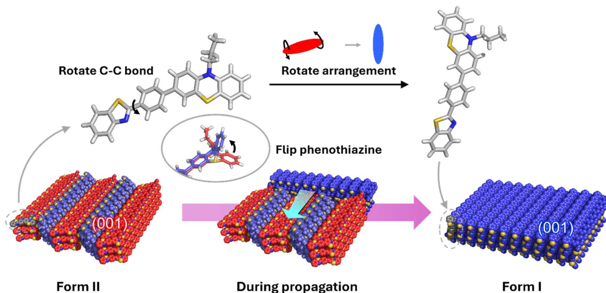
Fig. 5 Schematic illustration of the structural transition. During the transition, racemization by the flipping of phenothiazine, rotation of benzothiazole, and drastic changes in the molecular arrangement occurred.
