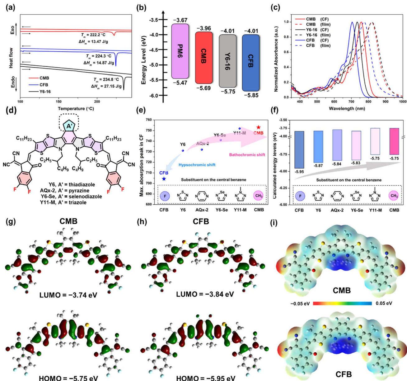
Fig. 2 (a) DSC measurements of CMB, Y6-16 and CFB with a ramping rate of 10\text{ }^\circ\text{C min}^{-1} . (b) Energy levels diagram of PM6, CMB, Y6-16 and CFB estimated by cyclic voltammetry. (c) Normalized absorption spectra of CMB, Y6-16 and CFB in chloroform and thin films. (d) General structure of Y6, AQx-2, Y6-Se and Y11-M. (e) Absorption \lambda_{\text{max}} of o -BDP-based NFAs in chloroform. (f) Trend of the calculated HOMO level of o -BDP-based NFAs. HOMO/LUMO distribution of (g) CMB and (h) CFB. (i) Electrostatic potential distribution diagram of CMB and CFB.
