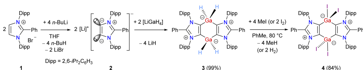
Scheme 1 Synthesis of \text{Ga}(\text{III}) hydride 3 and iodide 4 .
