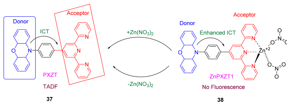
Fig. 15 Proposed mechanism for regulation of TADF using \text{Zn}^{2+} . Reproduced from ref. 159, https://doi.org/10.1039/C8SC01485J , under the terms of the CC BY-NC 3.0 license, https://creativecommons.org/licenses/by-nc/3.0/ .
