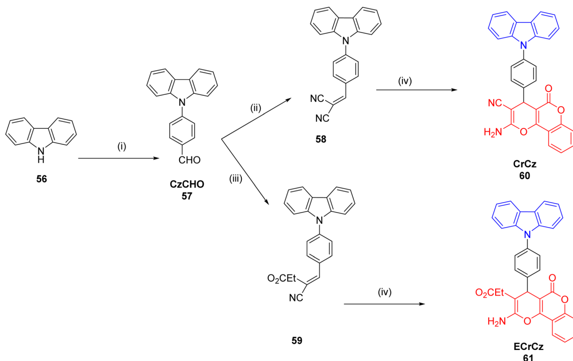
Fig. 42 Synthesis of CrCz and ECrCz starting from 9H-carbazole: (i) 4F-Ph-CHO, \text{K}_2\text{CO}_3 , N,N -dimethylformamide (DMF), 130 °C (ii) \text{CH}_2(\text{CN})_2 , EtOH, reflux; (iii) ethyl cyanoacetate, EtOH, reflux; (iv) 4-hydroxycoumarin, Ni-Np, EtOH. 207
