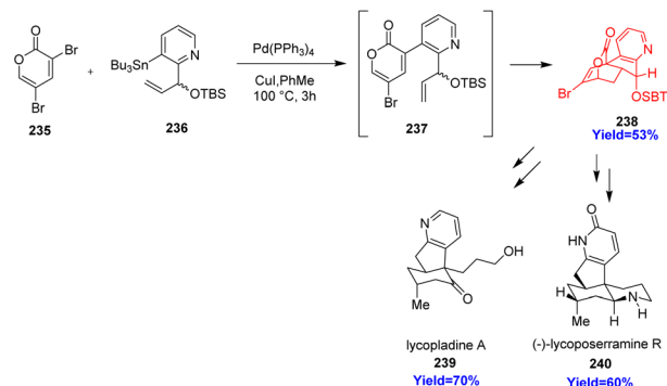
Scheme 30 Stille coupling between (235) and (236) accompanied with IMDA reaction produced (238) which further can be converted to the lycopoladine A (239) and (–)-lycopoloserramine R (240). 72
