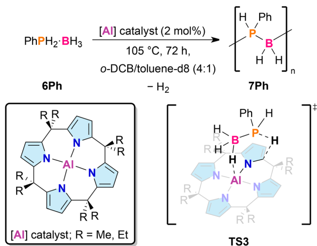
Fig. 4 Dehydrocoupling of \text{PhPH}_2\text{-BH}_3 using calix[4]pyrrolato aluminate as a catalyst. The proposed intermediate where P–H bond is acidified via a B–H–Al interaction ( TS3 ) is also shown.
