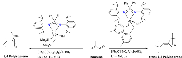
Scheme 48 Regio- and stereoselective isoprene polymerization using iminophosphoramidate-stabilized lanthanide complexes. 123
