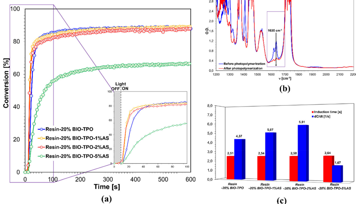
Fig. 6 Results achieved during radical photopolymerization of photocurable resins based on Resin-20%BIO-TPO with different amounts of the amine synergist AS during VisLED@405 nm diode irradiation under atmospheric oxygen-limited conditions: (a) kinetic profiles representing the time dependence of functional group conversion, (b) FT-IR spectrum before and after the radical photopolymerization process, including the band characteristic of C=C bonds, and (c) diagram illustrating the values of the kinetic curve slope and induction time obtained during radical photopolymerization for resins with increasing amounts of the amine synergist AS.
