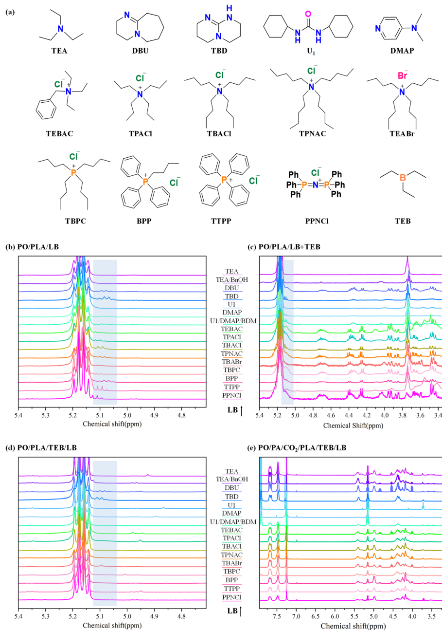
Fig. 3 (a) Schematic diagram of the structural formulas of Lewis bases and TEB. ^1\text{H} NMR spectra of (b) PO/PLA/LB at 70 °C for 2 h; (c) adding TEB into PO/PLA/LB at 70 °C for 2 h; (d) PO/PLA/TEB/LB at 70 °C for 2 h and (e) products resulting from the copolymerization of PO, PA, and \text{CO}_2 and PLA transesterification with TEB and different Lewis bases at 65 °C for 6 h.
