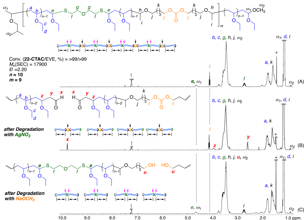
Fig. 3 ^1\text{H} NMR spectra ( \text{CDCl}_3 , 55\text{ }^\circ\text{C} ) of the obtained copolymer of EVE and 22-CTAC (A) and the polymers after degradation using an \text{AgNO}_3 solution (B) and using a \text{NaOCH}_3 solution (C): [\text{thioacetal unit}]_0/[\text{AgNO}_3]_0 = 5.0/50\text{ mM} in \text{THF}/\text{H}_2\text{O} at 20\text{ }^\circ\text{C} or [\text{carbonate unit}]_0/[\text{NaOCH}_3]_0 = 5.0/50\text{ mM} in \text{CH}_3\text{OH} at 60\text{ }^\circ\text{C} . *: \text{H}_2\text{O} , †: \text{CHCl}_3 .
