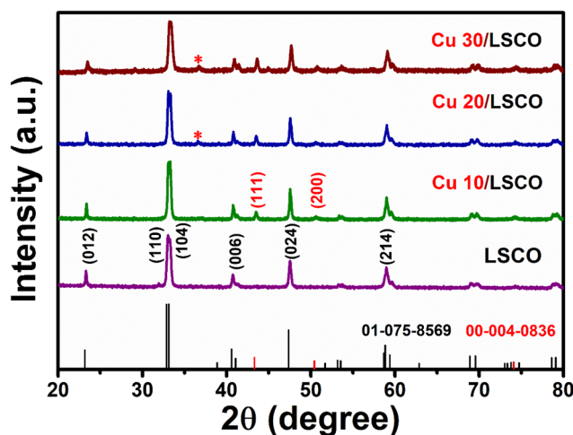
Fig. 1 Comparative X-ray diffraction patterns of crystalline LSCO, Cu 10/LSCO, Cu 20/LSCO and Cu 30/LSCO. The asterisks (*) denote the presence of the (111) plane of the Cu 2 O phase, distinct from the metallic Cu peaks. This comparison highlights the structural evolution and phase composition as a function of increasing copper content in the LSCO matrix.
