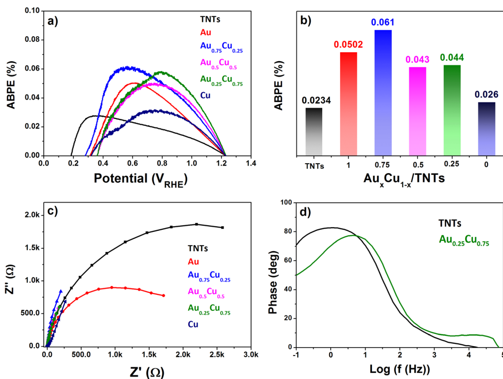
Fig. 8 (a) ABPE plot of all electrodes; (b) ABPE values at 0.6 V RHE ; (c) EIS spectra of pristine and AuCu x TNT (x = 1, 0.75, 0.5, 0.25 and 0) electrodes measured under AM 1.5G illumination; (d) Bode plot of pristine TNTs and Au 0.25 Cu 0.75 /TNTs, measured in 0.5 M Na 2 SO 4 at pH 7.2.
