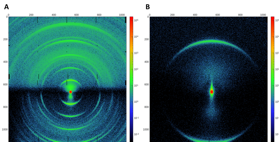
Fig. 3 (A) and (B) Two-dimensional grazing-incidence wide-angle (A) and small-angle (B) X-ray scattering patterns of a (\text{C}_6\text{H}_5\text{--CH}_2\text{--CH}_2\text{--NH}_3)_2\text{PbBr}_4 liquid crystal.
