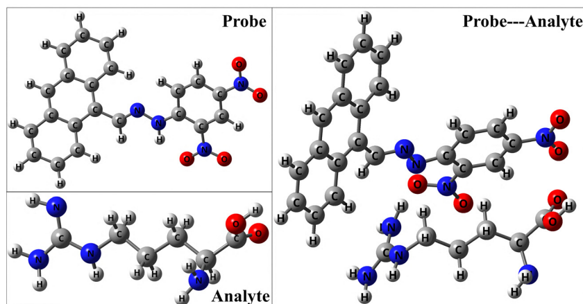
Fig. 8 Molecular geometries of the optimized probe ( P1 ), analyte ( A1 ), and the product ( P1 · A1 ) with atomic labelling of all atoms obtained at the CAM-B3LYP/6-31+G(d,p) level of theory using the CPCM-DMSO solvation model.
