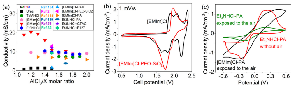
Fig. 15 (a) Ionic conductivity of various \text{AlCl}_3/\text{X} electrolytes. \text{X} = [\text{EMIm}]\text{Cl} ( 10\text{--}20\text{ mS cm}^{-1} ), TMAHCl (average \sim 7.5\text{ mS cm}^{-1} ), \text{Et}_3\text{NHCl} ( \sim 9.6\text{ mS cm}^{-1} ), [\text{BMIm}]\text{Cl} ( \sim 9.4\text{ mS cm}^{-1} ), and urea ( \sim 1.3\text{ mS cm}^{-1} ) were measured at 25^\circ\text{C} . 98 [\text{EMIm}]\text{Cl-PA} ( 1.66 \times 10^{-3}\text{ S cm}^{-1} , measured at 20^\circ\text{C} ) is gel polymer electrolyte made from PEO, \text{AlCl}_3/[\text{EMIm}]\text{Cl} (1.5 : 1) and an additive-fumed \text{SiO}_2 . 2 [\text{EMIm}]\text{Cl-PA} (5.89 to 7.24\text{ mS cm}^{-1} , measured at room temperature) and \text{Et}_3\text{NHCl-PA} ( 3.86\text{ mS cm}^{-1} , measured at 25^\circ\text{C} ) is PA-based gel polymer electrolyte made with \text{AlCl}_3/[\text{EMIm}]\text{Cl} (2 : 1 to 1.3 : 1) 138 and \text{AlCl}_3/\text{Et}_3\text{NHCl} (1.7 : 1), 139 respectively. \text{AlCl}_3/\text{Et}_3\text{NHCl} (1.5 : 1) add CTAC ( 12.06\text{ mS cm}^{-1} ) 33 and F127 ( 9.31\text{ mS cm}^{-1} ) 32 are named \text{Et}_3\text{NHCl} + \text{CTAC} and \text{Et}_3\text{NHCl} + \text{F127} , respectively. (b) CV curves of Al/natural graphite cells with \text{AlCl}_3/[\text{EMIm}]\text{Cl} and \text{AlCl}_3/[\text{EMIm}]\text{Cl-PEO-SiO}_2 electrolytes showing anions intercalation at a scan rate of 1\text{ mV s}^{-1} . Adapted from Leung, O. M. et al., Adv. Energy Mater. 2 Licensed under CC BY 3.0. ©2024 John Wiley and Sons. (c) CV curves of Al/natural graphite cells with \text{AlCl}_3/[\text{EMIm}]\text{Cl-PA} 138 (not mentioning the scan rate) and \text{AlCl}_3/\text{Et}_3\text{NHCl-PA} 139 (without air not mentioning the scan rate, and after being exposed to the air for 10 min at a scan rate of 1\text{ mV s}^{-1} ) presenting Al plating/stripping. Adapted with permission from Elsevier. 138 Copyright 2021. Adapted with permission from American Chemical Society. 139 Copyright 2021.
