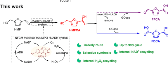
Scheme 1 The previous and current strategies for the selective synthesis of HMFA, FFCA and FDCA. (A) Previous study. (B) This work.
