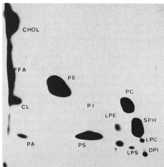
Fig. 3 2D TLC of MeOH then \text{CHCl}_3 extraction of red blood cell lipids showing each phospholipid. Originally Fig. 3 of Roelefsen & Zwaal 1976. 18 By phosphate assay of each scraped spot 17 quantitation is achieved.
