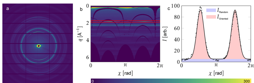
Fig. 2 Orientation analysis. Raw detector frame (a). Azimuthally resolved detector frame after integration. The red box indicates the (002) peak, which shows the c-axis orientation of the apatite crystallites (b). Local background subtracted (002) orientation signal. The dots show the data, line shows fit. The position of the peak gives the orientation, the ratio I_{\text{oriented}}/(I_{\text{oriented}} + I_{\text{random}}) gives the DoO and the total signal is the sum of the red and blue areas (c).
