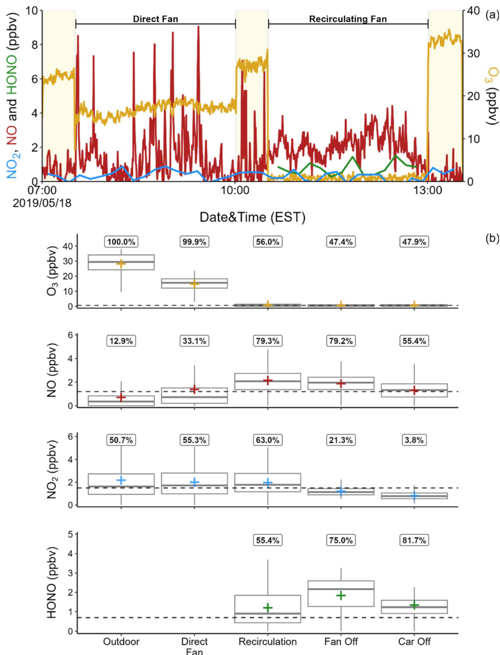
Fig. 1 (a) Representative time series for NO, \text{NO}_2 , HONO, and \text{O}_3 over 7 hours of measurements. Light yellow shaded regions represent outdoor measurements. (b) Box-and-whiskers plot for analyte concentrations under indoor and outdoor conditions. Box plots display quartile values and medians. Whiskers extend to the minimum and maximum values within 1.5 times the interquartile range. Crosses represent the mean value for each condition. Horizontal dashed lines represent the LOD for each species, and percentages above the violin plots represent the fraction of measurements above the LOD. Nitrous acid concentrations under outdoor and direct fan conditions are not reported due to a sampling artefact.
