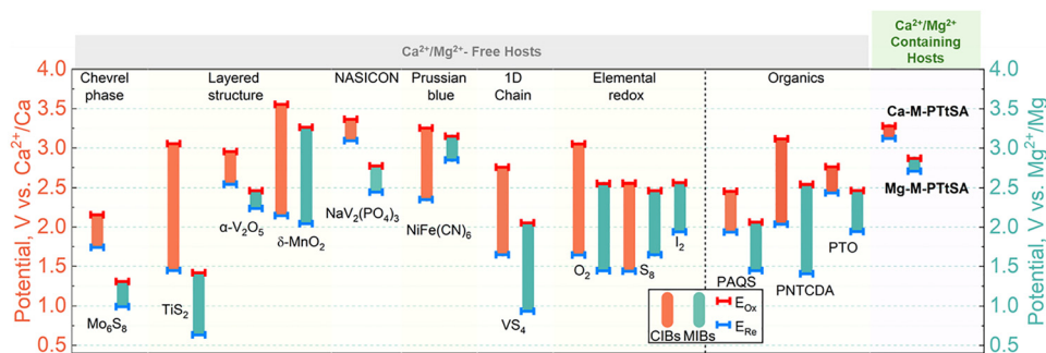
Fig. 1 Electrochemical characteristics of state-of-the-art divalent positive electrode materials. Comparison of DI-M-PTSA materials developed in this work with leading materials studied to date for \text{Mg}^{2+} and \text{Ca}^{2+} storage, based on average oxidation–reduction potential values and hysteresis (the details of comparison analysis are given in Table S1). Legend: CIBs, calcium-ion battery materials; MIBs, magnesium-ion battery materials; E_{\text{ox}} , average oxidation potential; E_{\text{red}} , average reduction potential.
