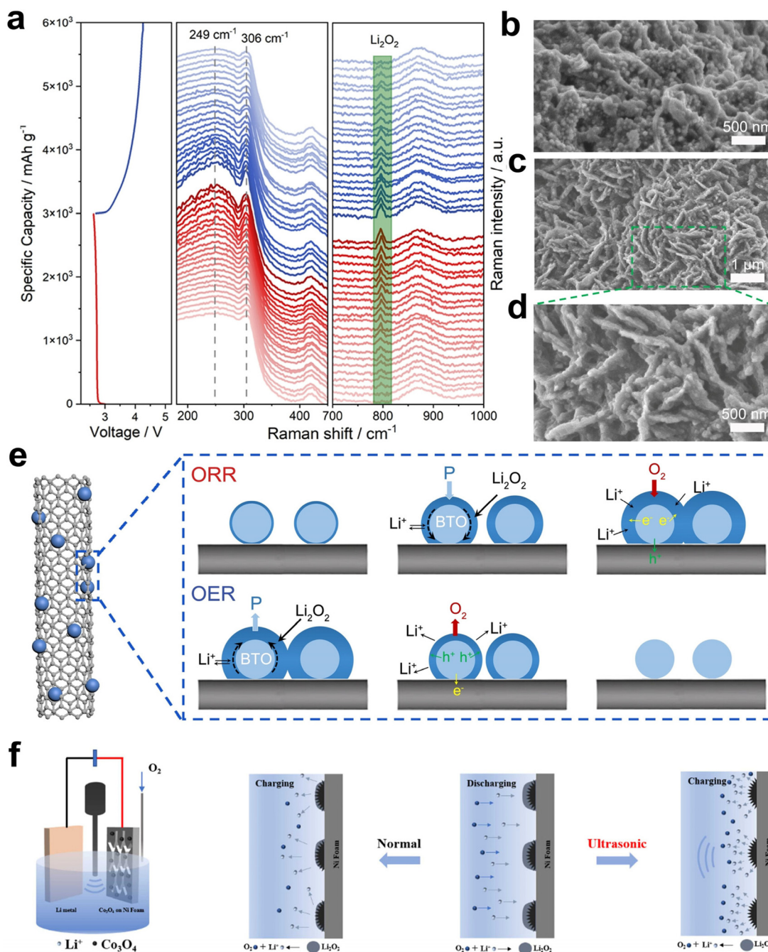
Fig. 16 (a) In situ electrochemical Raman spectra collected on the BTO-CNT cathode at a current density of 300 mA g -1 . (b) SEM image of the BTO-CNT cathode at a discharge depth of 1500 mA h -1 and a current density of 300 mA g -1 . (c and d) Low- and high-magnification SEM images of the BTO-CNT cathode at a discharge depth of 3000 mA h -1 under a current density of 300 mA g -1 . (e) Schematic illustration of Li 2 O 2 formation and decomposition on the BTO surface. 169 (f) Schematic diagram of the ultrasonic charging mechanism on the electrode surface. 180
