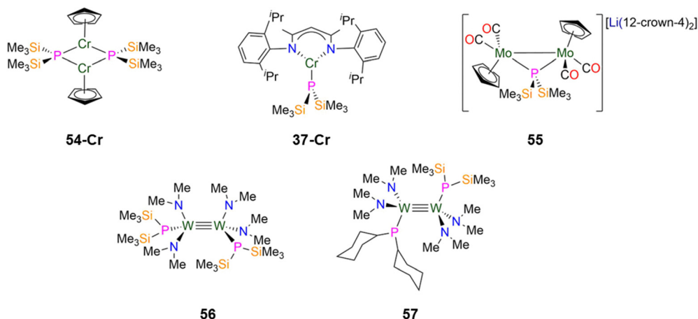
Fig. 15 Group 6 P'' complexes [\text{Cr}(\text{Cp})(\mu\text{-P}'')_2] ( 54-Cr ), [\text{Cr}(\text{DippPnacnac})(\text{P}'')] ( 37-Cr ; \text{DippPnacnac} = \text{CH}\{(\text{CH}_3)_2\text{CN}(\text{Dipp})\}_2 ; \text{Dipp} = \text{C}_6\text{H}_3\text{Pr}_2\text{-2,6} ), [\text{Li}(12\text{-crown-4})][\{\text{Mo}(\text{Cp})(\text{CO})_2(\mu\text{-P}'')\}] ( 55 ), [\text{1,2-W}_2(\text{P}'')(\text{NMe}_2)_4] ( 56 ), [\text{1,2-W}_2(\text{PCy}_2)(\text{P}'')(\text{NMe}_2)_4] ( 57 ).
