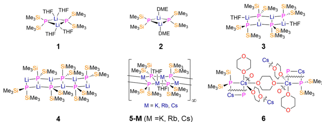
Fig. 2 Group 1 M'' complexes [\text{Li}(\mu\text{-P}'')(\text{THF})_2]_2 ( 1 ), [\text{Li}_4(\mu_2\text{-P}'')_2(\mu_3\text{-P}'')_2(\text{THF})_2] ( 2 ), [\text{Li}(\mu\text{-P}'')(DME)_2]_2 ( 3 ), [\text{Li}_6(\mu_2\text{-P}'')_2(\mu_3\text{-P}'')_4] ( 4 ), [\text{M}_4(\mu_2\text{-P}'')_2(\mu_3\text{-P}'')_2]_\infty ( 5-M ; M = \text{K, Rb, Cs} ), [\text{Cs}(\mu\text{-P}'')(\mu\text{-1,4-dioxane})_3(1,4\text{-dioxane})]_\infty ( 6 ).
