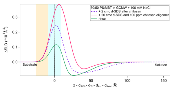
Fig. 12 Subtracted SLD profiles of a pre-mixed d25-SDS/chitosan complex adsorbed on 50 : 50 MBT : PS (magenta line), and the following rinse (green). For comparison, the profile corresponding to the same molecules adsorbed in successive steps (same as Fig. 8) is added (dashed line). The zero of the x -axis is at the thiol/d25-SDS interface, whose roughness is indicated by the blue panel. Similarly, the yellow panel on the left represents the Au/thiol interface with its associated roughness.
