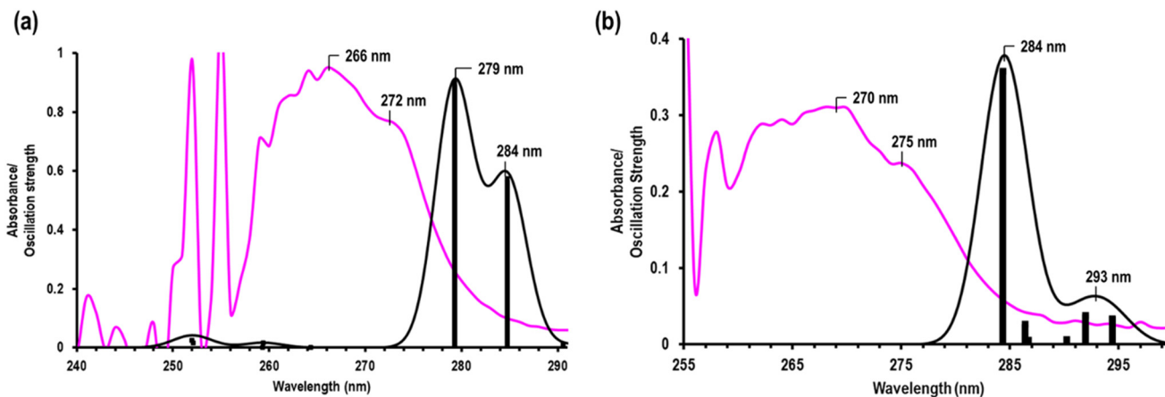
Fig. 13 B3LYP TDDFT-computed oscillators (bars) using MeCN and DMSO as solvents, overlaid with Gaussian broadening curves (black) and the experimental UV-visible spectra (magenta) of Ag(2,3-Lut) 2 (NO 3 ) in MeCN (a) and Ag(3-Brpy) 3 (NO 3 ) in DMSO (b).
