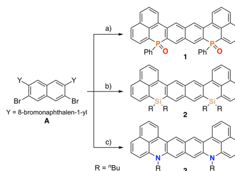
Scheme 1 Reaction conditions for the synthesis of hexaarenes 1 , 2 and 3 . Conditions: (a) 1. t BuLi, -80\text{ }^\circ\text{C} ; 2. \text{PhPCl}_2 ; 3. \text{H}_2\text{O}_2 . (b) 1. t BuLi, -80\text{ }^\circ\text{C} ; 2. {}^n\text{Bu}_2\text{SiCl}_2 . (c) \text{Pd}_2(\text{dba})_3 , R -BINAP, \text{NaO}^t\text{Bu} , t BuNH 2 .
