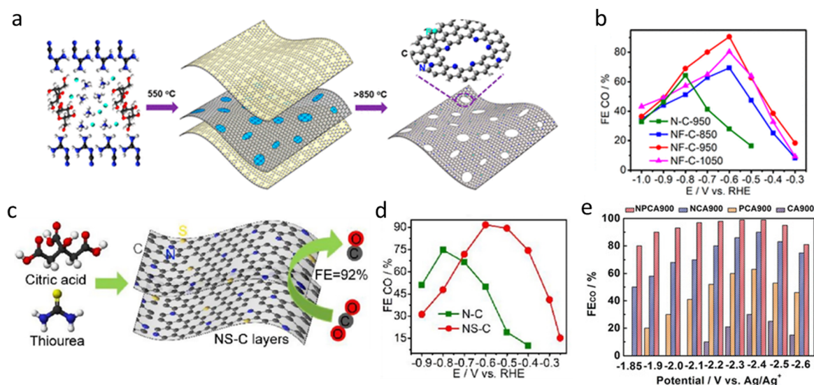
Fig. 4 (a) and (b) Schematic illustration of the processing for the synthesis of holey NF-C layers; FE_{CO} of N-C and NF-C at different pyrolysis temperatures. 97 Reprinted with permission. Copyright 2019 American Chemical Society. (c) and (d) Schematic of NS-C synthesis; CO Faraday efficiency of N-C and NS-C. 98 Reproduced with permission. Copyright 2019 Elsevier. (e) The FE_{CO} for NPCA900, NCA900, PCA900 and CA900 at different applied potentials. 99 Reprinted with permission. Copyright 2020 Wiley.
