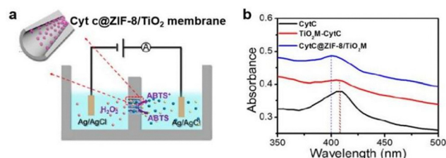
Fig. 11 (a) Schematic illustration of \text{Cyt c@ZIF-8/TiO}_2 membrane in electrocatalysis cell and its working mechanism. (b) UV-Vis diffuse reflectance spectra of CytC (black), \text{TiO}_2 membrane-CytC (red), and \text{Cyt c@ZIF-8/TiO}_2 membrane (blue) with high-purity \text{BaSO}_4 employed as the background. Reproduced with permission from ref. 60.
