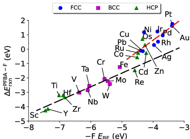
Fig. 6 \Delta E_{\text{rxn}}^{\text{PFBA-F}} vs. fluorine binding for the removal of a -F from a C_\alpha carbon on transition metal surfaces. The black dashed line represents a linear fit to the data for the carbo binding mode ( \Delta E_{\text{rxn}}^{\text{PFBA-F}} = 0.95E_{\text{BE}} - F + 3.09 , R^2 = 0.92 ). The red dashed line represents a linear fit to the flat binding mode ( \Delta E_{\text{rxn}}^{\text{PFBA-F}} = 1.59E_{\text{BE}} - F + 6.98 , R^2 = 0.67 ).
