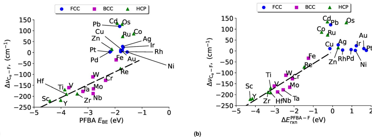
Fig. 7 C_\alpha -F vibrational shifts ( \Delta\nu_{C_\alpha-F} ) vs. (a) PFBA binding ( E_{\text{BE}}^{\text{PFBA}} ) and (b) \Delta E_{\text{rxn}}^{\text{PFBA-F}} on transition metal surfaces. The black dashed line represents a linear fit to the data for the carbo binding mode: (a) \Delta\nu_{C_\alpha-F} = 28.86E_{\text{BE}}^{\text{PFBA}} + 58.64 , R^2 = 0.73 and (b) \Delta\nu_{C_\alpha-F} = 55.21\Delta E_{\text{rxn}}^{\text{PFBA-F}} - 2.53 , R^2 = 0.82 . No stable solution exists for the linear regression of the flat binding mode.
