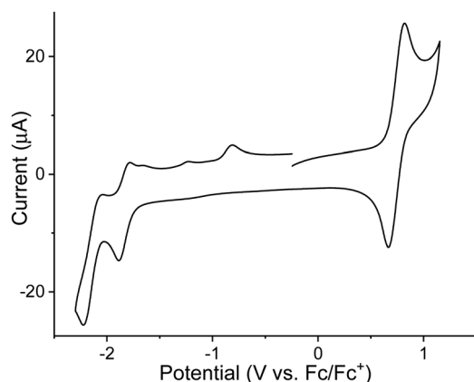
Fig. 2 Cyclic voltammetry for compound 1 in 1,2-dichlorobenzene solution (ca. 10^{-5} M), in the presence of 10^{-1} M (n\text{-Bu}_4\text{N})(\text{PF}_6) as a supporting electrolyte measured at a scan rate of 100 \text{ mV s}^{-1} .
