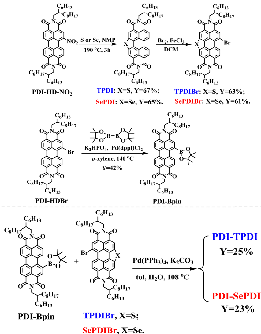
Scheme 1 Synthesis of monobromides TPDI-Br and SeTPDI-Br , monoboric ester PDI-Bpin and asymmetric PDI dimeric acceptors PDI-TPDI and PDI-SeTPDI .
