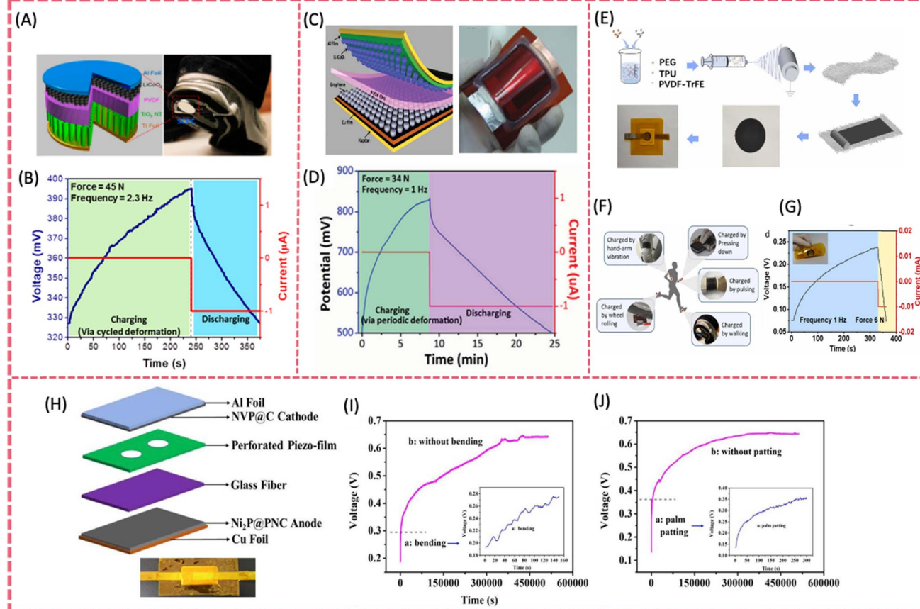
Fig. 9 (A) Structure and applications of a SCPC made of LiCoO 2 (cathode) and TiO 2 (anode) separated using a polarized PVDF membrane and (B) self-charging process under compressive force. Reproduced from ref. 17 with permission from American Chemical Society, copyright 2012. (C) Structure and optical image of the flexible SCPC made of LiCoO 2 (cathode) and graphene nanosheet composites (anode) separated using a polarized PVDF film and (D) self-charging process of the flexible SCPC under compressive force. Reproduced from ref. 129 with permission from Wiley-VCH GmbH, copyright 2014. (E) Fabrication procedure of the fully flexible SCPC; (F) possible applications of the SCPC to utilize biomechanical energy and (G) self-charging response of the fully flexible SCPC. Reproduced from ref. 128 with permission from Elsevier, copyright 2022. (H) Device architecture of the flexible SC SIB; (I) self-charging process by bending and (J) palm patting. Reproduced from ref. 24 with permission from Elsevier, copyright 2019.
